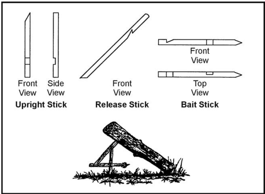
Figure 8-13. Figure 4 Deadfall
