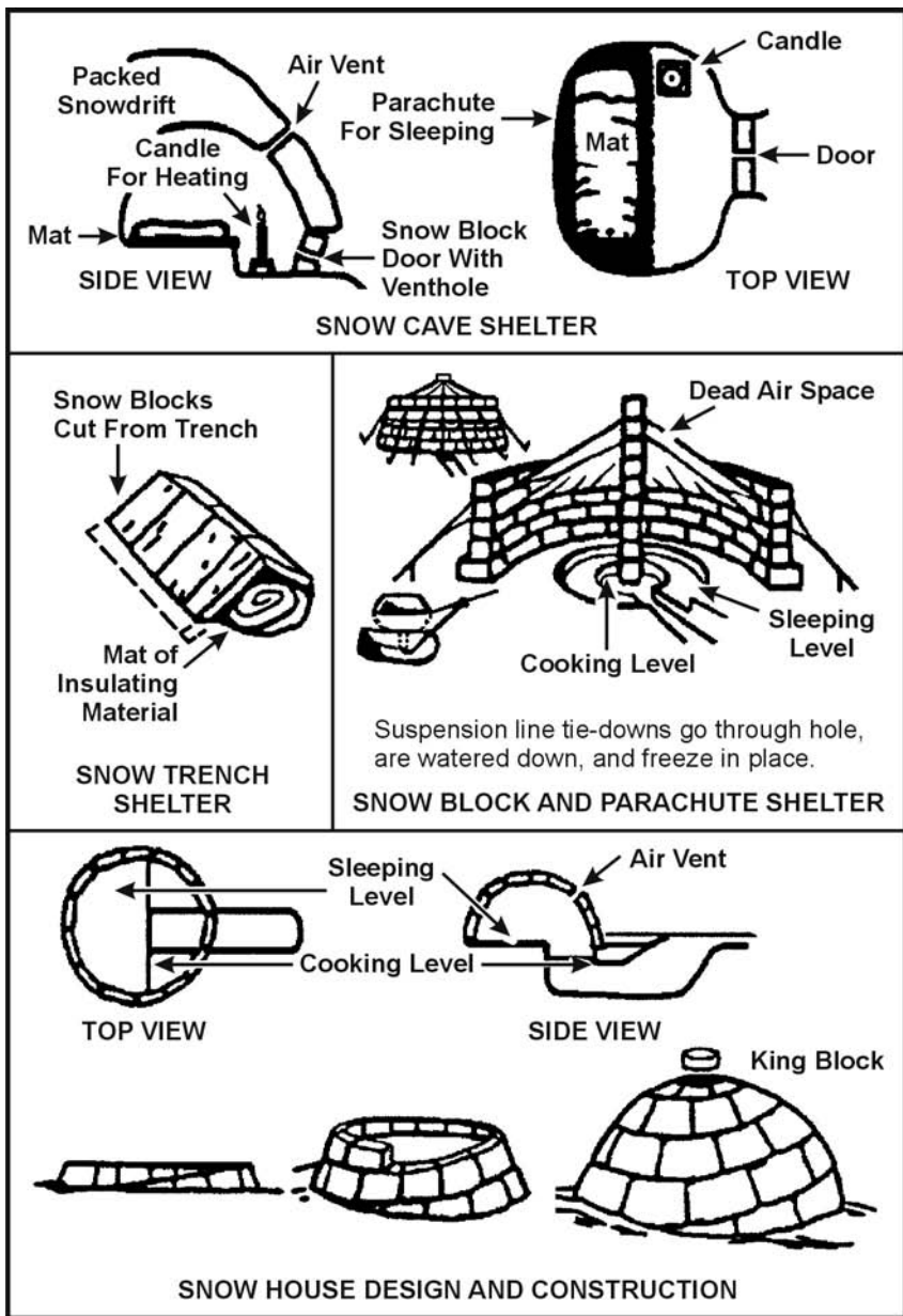
Figure 15-4. Snow Dwellings
