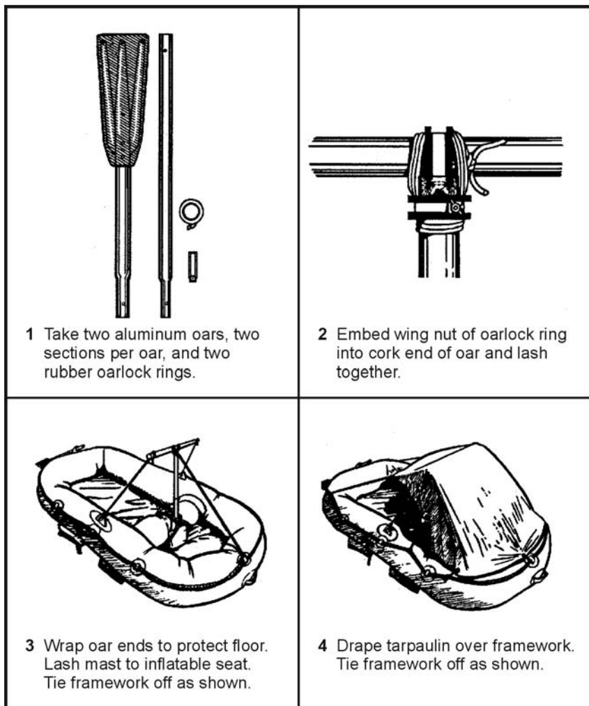
Figure 16-17. Sail Construction
