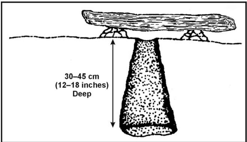
Figure 8-17. Bottle Trap
