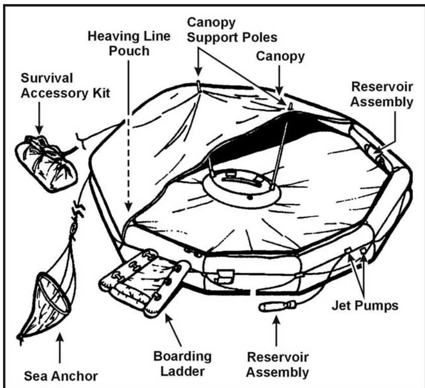
Figure 16-15. 25-Man Raft
