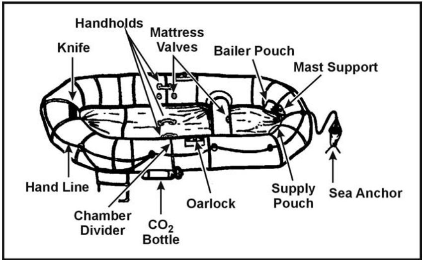
Figure 16-12. Seven-Man Raft
