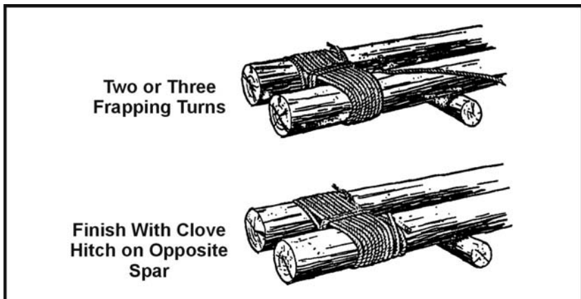
Figure G-14. Shears Lashing
