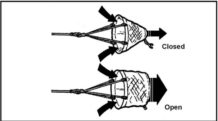
Figure 16-5. Sea Anchor
