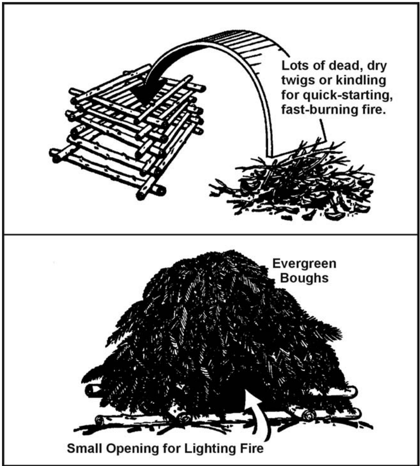
Figure 19-2. Smoke Generator—Ground
