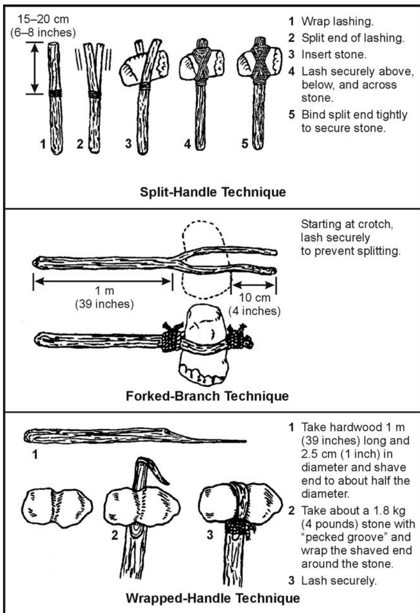
Figure 12-1. Lashing Clubs
