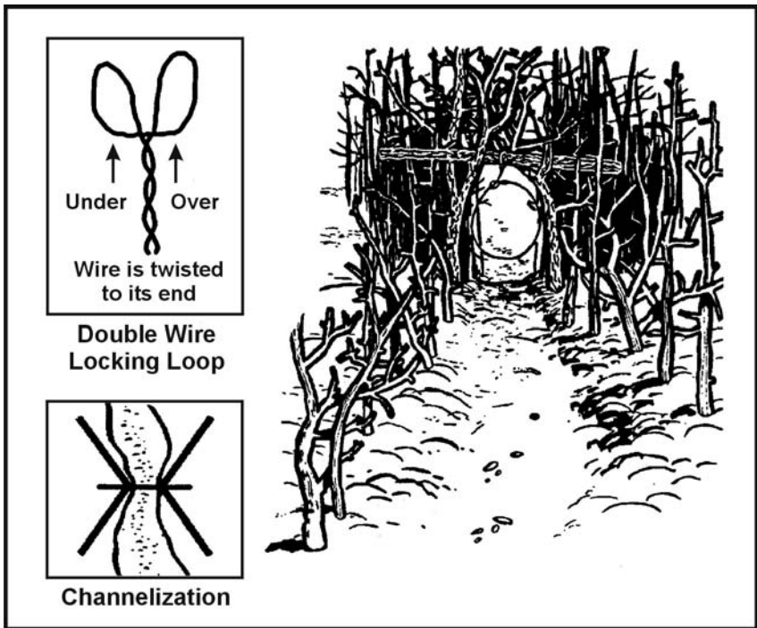
Figure 8-7. Drag Noose
