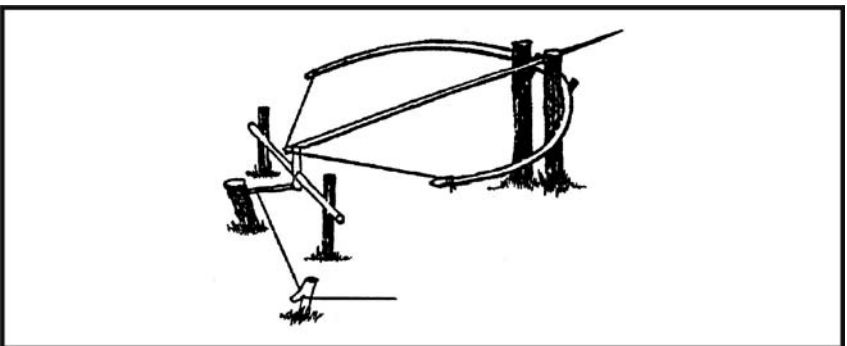
Figure 8-15. Bow Trap
